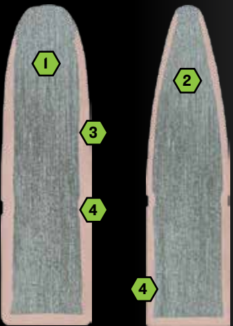
CORE-LOKT SOFT POINT CORE-LOKT POINTED SOFT POINT
